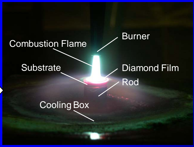
Synthesizing diamond on the substrate by the combustion flame.
