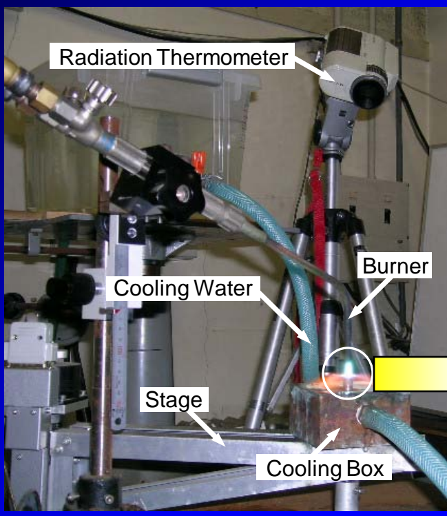
Experimental setup for synthesizing diamond by acetylene-oxygen combustion flame.
