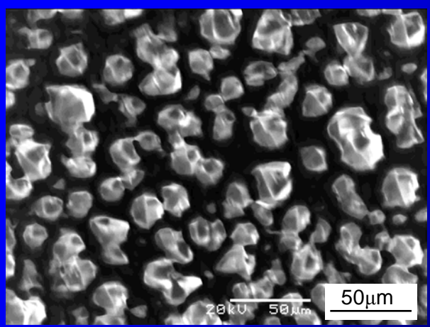
SEM image of synthesized diamond film that the delamination was prevented.
